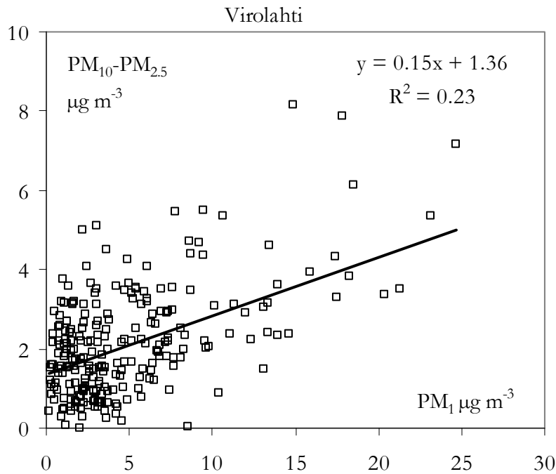
Figure 20. Mass concentration of coarse particle mode as a function of accumulation mode at Virolahti. PM 10 and PM 2.5 were sampled using filter technique.
