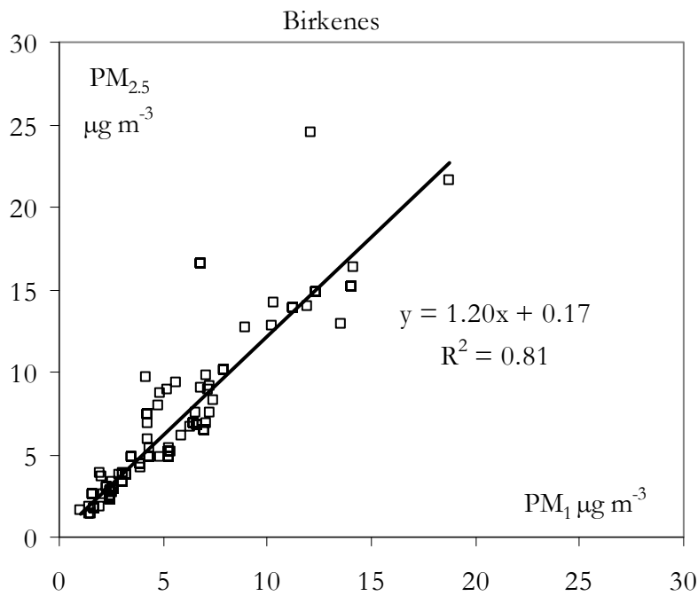
Figure 22. Mass concentration of PM 2.5 (filter sampling) as a function of PM 1 when all PM x data have been reasonable at Birkenes.
