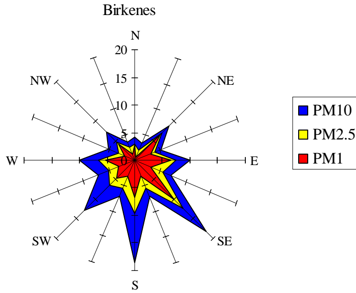
Figure 10. Average PM_1 , PM_{2.5} and PM_{10} concentrations ( \mu g m^{-3} ) at Birkenes, when data for all three PM -fractions are available and reasonable simultaneously, as a function of sector for the wind trajectory.
