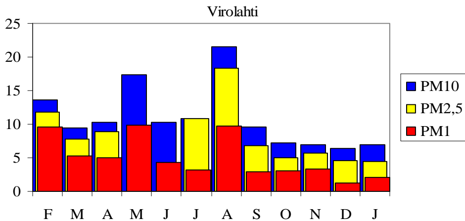
Figure 16. Average PM 1 , PM 2.5 and PM 10 concentrations (µg m -3 ) at Virolahti.
