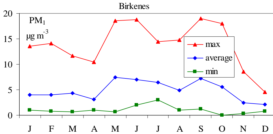
Figure 5. Minimum, average and maximum PM 1 concentrations at Birkenes.
