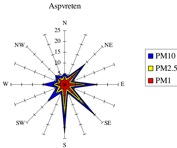
Figure 11. Average PM_1 , PM_{2.5} and PM_{10} concentrations ( \mu g m^{-3} ) at Aspvreten, when data for all three PM -fractions are available and reasonable simultaneously, as a function of sector for the wind trajectory.
