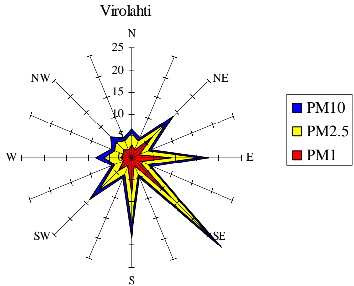
Figure 12. Average PM 1 , PM 2.5 and PM 10 concentrations ( \mu\text{g m}^{-3} ) at Virolahti, when data for all three PM-fractions are available and reasonable simultaneously, as a function of sector for the wind trajectory.
