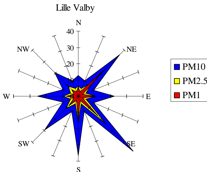
Figure 9. Average PM 1 , PM 2.5 and PM 10 concentrations ( \mu\text{g m}^{-3} ) at Lille Valby, when data for all three PM-fractions are available and reasonable simultaneously, as a function of sector for the wind trajectory.
