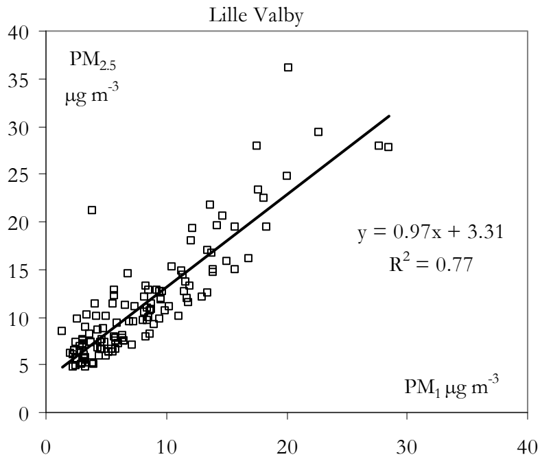
Figure 21. Mass concentration of PM 2.5 (TEOM) as a function of PM 1 when all PM x data are reasonable at Lille Valby.
