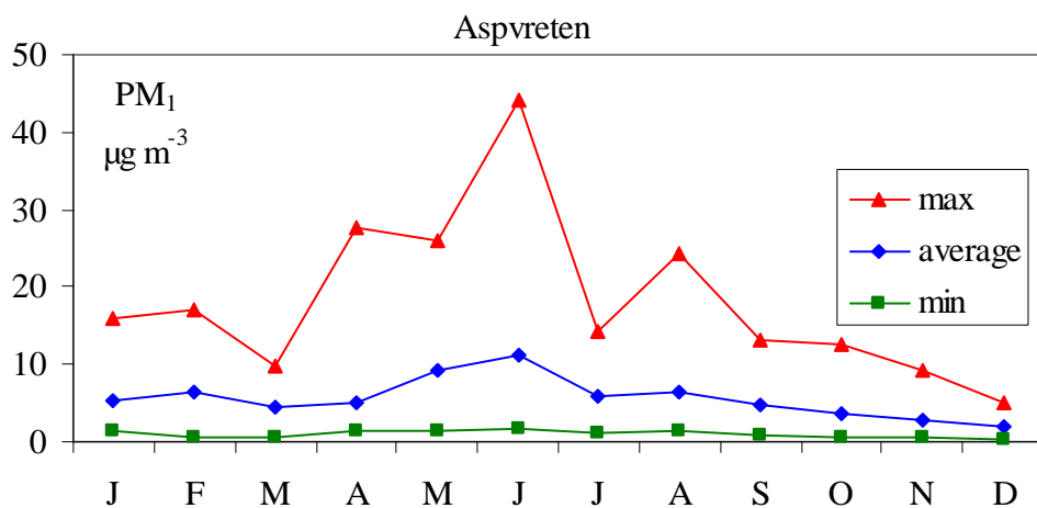
Figure 6. Minimum, average and maximum PM 1 concentrations at Aspvreten.
