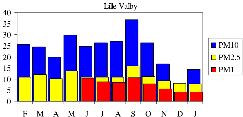
Figure 13. Average PM 1 , PM 2.5 and PM 10 concentrations ( \mu\text{g m}^{-3} ) at Lille Valby.
