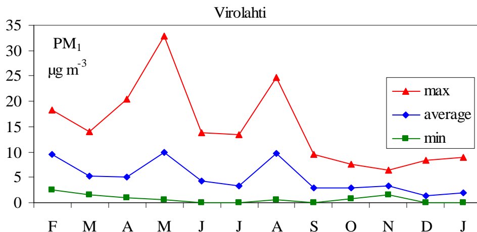
Figure 7. Minimum, average and maximum PM 1 concentrations at Virolahti.
