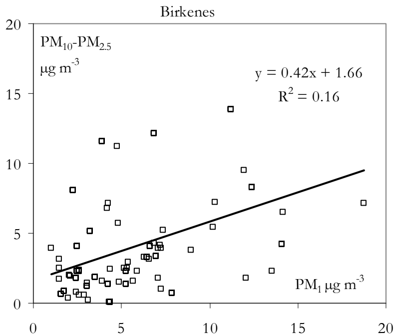
Figure 18. Mass concentration of coarse particle mode as a function of accumulation mode at Birkenes. PM 10 and PM 2.5 were both measured using filter sampling.
