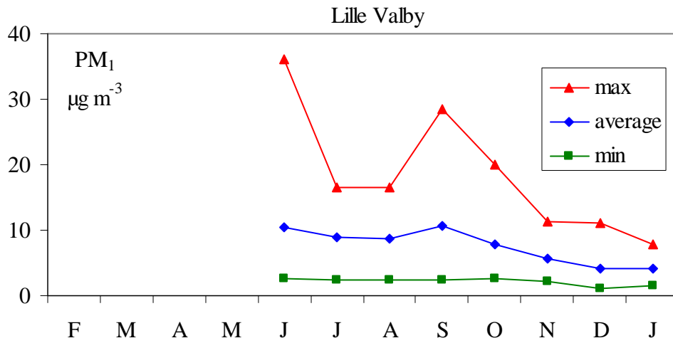
Figure 4. Minimum, average and maximum PM 1 concentrations at Lille Valby.
