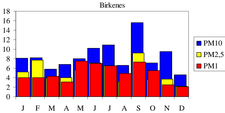
Figure 14. Average PM 1 , PM 2.5 and PM 10 concentrations (µg m -3 ) at Birkenes.
