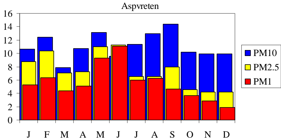
Figure 15. Average PM 1 , PM 2.5 and PM 10 concentrations (µg m -3 ) at Aspveten.
