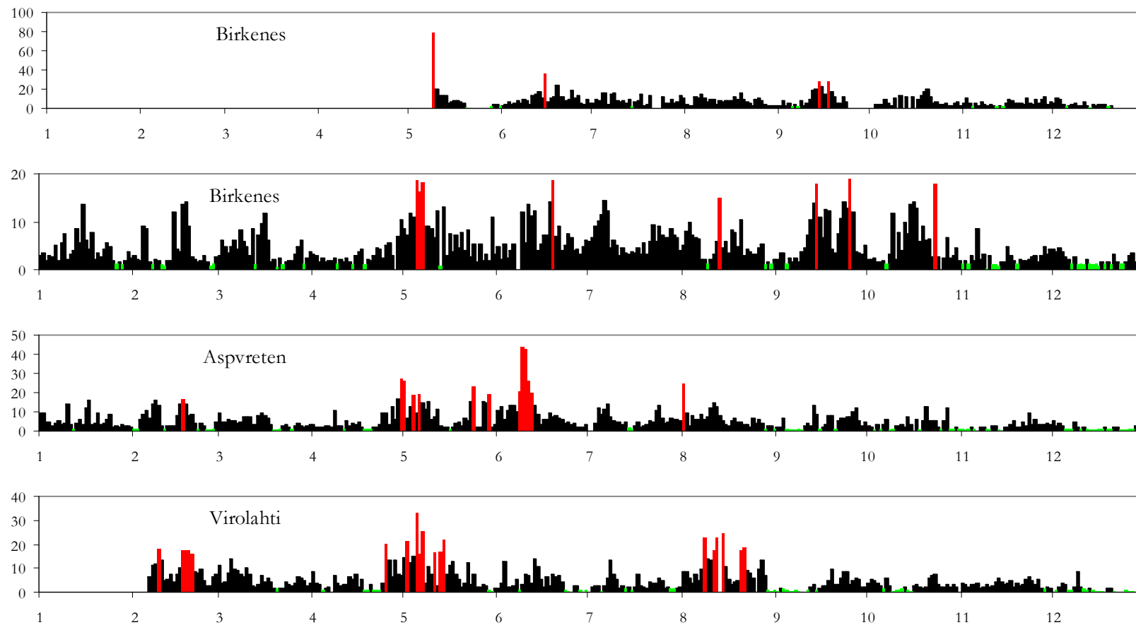
Figure 8. PM 1 concentrations during 2006. The numbers mark the starting point of each month. Red bars represent daily concentrations exceeding the annual average by a factor of three, whereas the green bars show daily concentrations less than 30 % of the annual average concentration.
