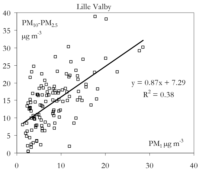
Figure 17. Mass concentration of coarse particle mode as a function of accumulation mode at Lille Valby. ( PM_{10} was measured with beta attenuation monitor and PM_{2.5} with TEOM).
