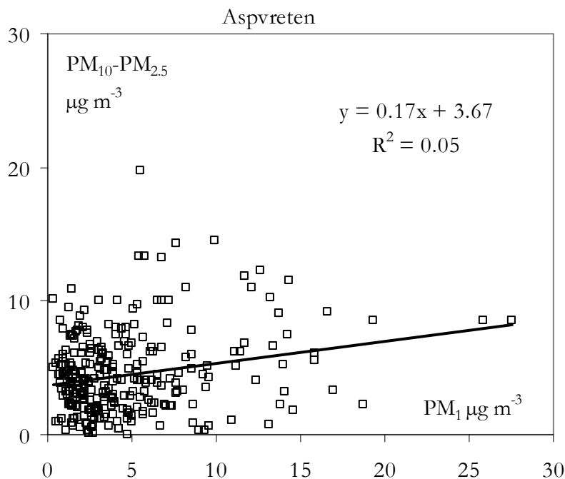
Figure 19. Mass concentration of coarse particle mode as a function of accumulation mode at Aspvreten. PM 10 was measured with TEOM and PM 2.5 using filter sampling.
