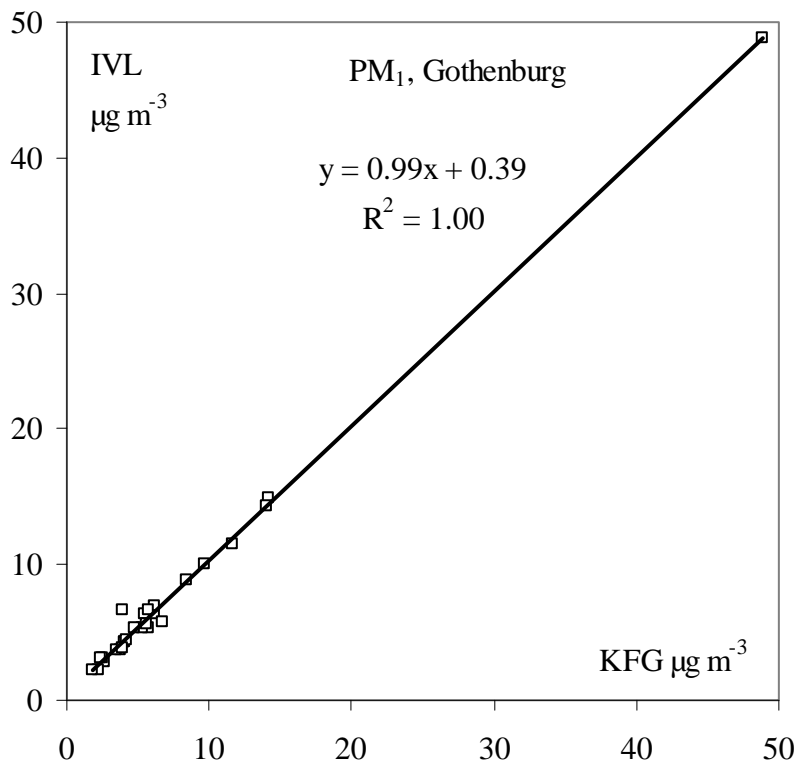
Figure 3. Scatter plot showing concentrations of PM 1 in an urban environment obtained using the IVL-head (inlet) and the reference method. (KFG = Kleinfiltergerät).
