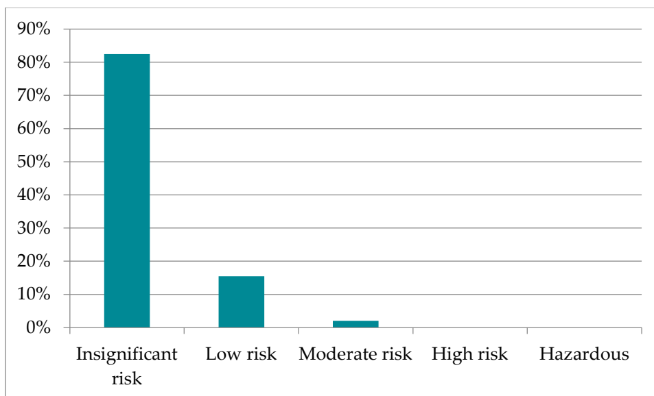
Figure 3: Outcome of the environmental risk assessments of pharmaceuticals at Fass.se (n = 97).
