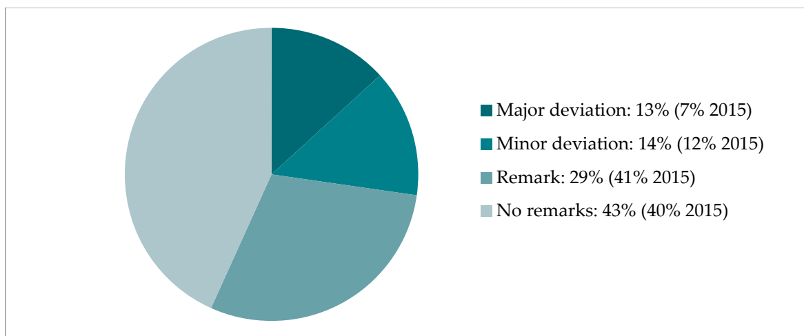
Figure 1: Distribution of the highest grade of recommendations that each company received for a specific substance that was sent in for review during 2016. The figure is based on the total number of reviews, i.e. 450 and the figure shows the highest grade of comment for each risk assessment during the year in the order: major deviation > minor deviation > remark > no remarks.
