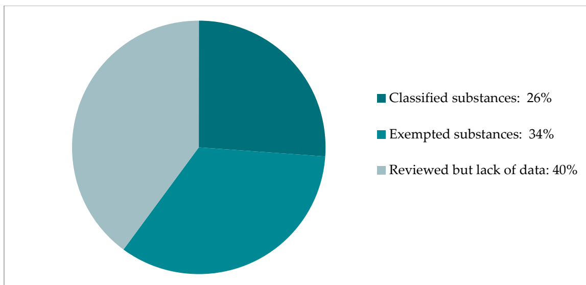
Figure 2: Outcome in terms of environmental classification of substances at Fass.se (n = 371). The figure covers classification of environmental risk, i.e. not potential for degradation or bioaccumulation.
