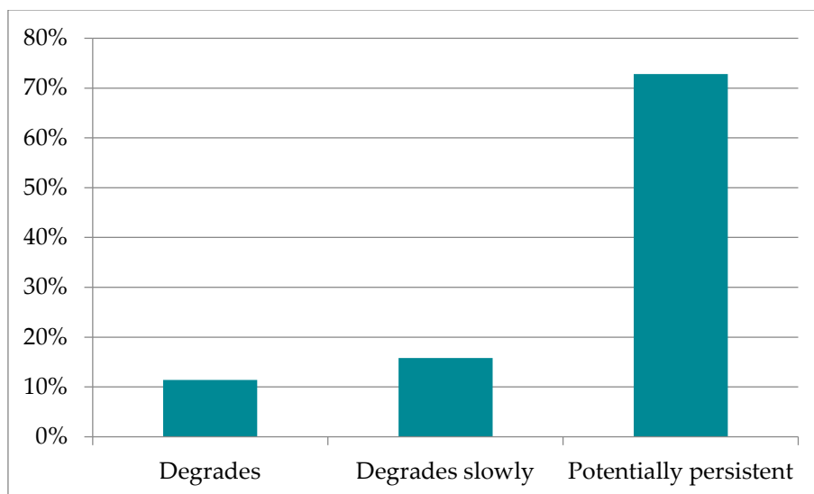
Figure 5: Outcome of the classification of degradation at Fass.se for documents published during 2016 (n = 114).
