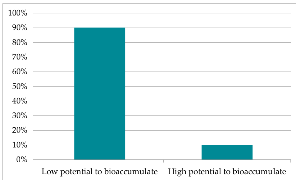
Figure 4: Outcome of the classification of bioaccumulation at Fass.se (n = 224).
